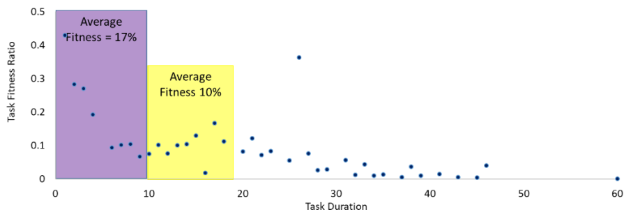
Figure 2: Task Fitness in CSD based on ACO
