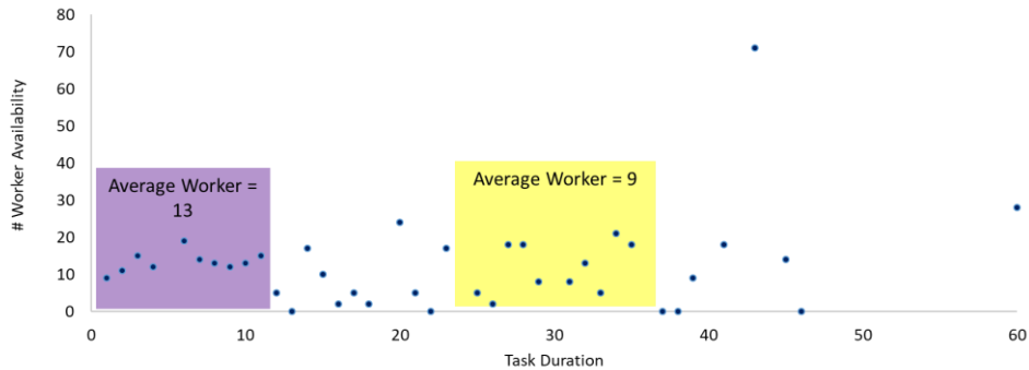
Figure 3: Distribution of Workers' Attraction in CSD base on ACO
